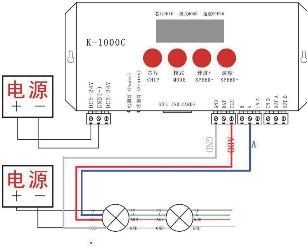
DMX512 single line signal wiring diagram: A(DAT)/ADD/GND
